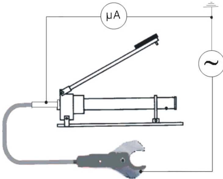
Fig. 4 The system for measuring the leakage current
